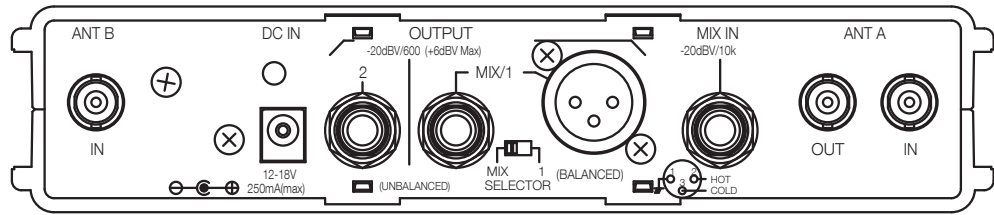
Rear View
