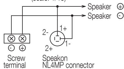
Wiring Diagram
