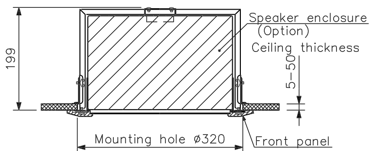
Ceiling Mounting
