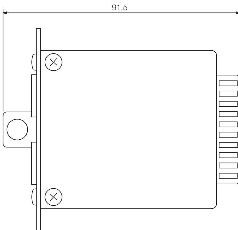
Side View
