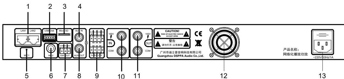
MAG6806/MAG6812 Rear Panel
